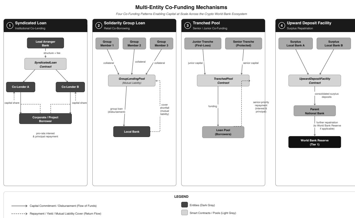
Figure 1.4: Multi-entity co-funding mechanisms: syndicated loan, solidarity group, tranched pool, and upward deposit
