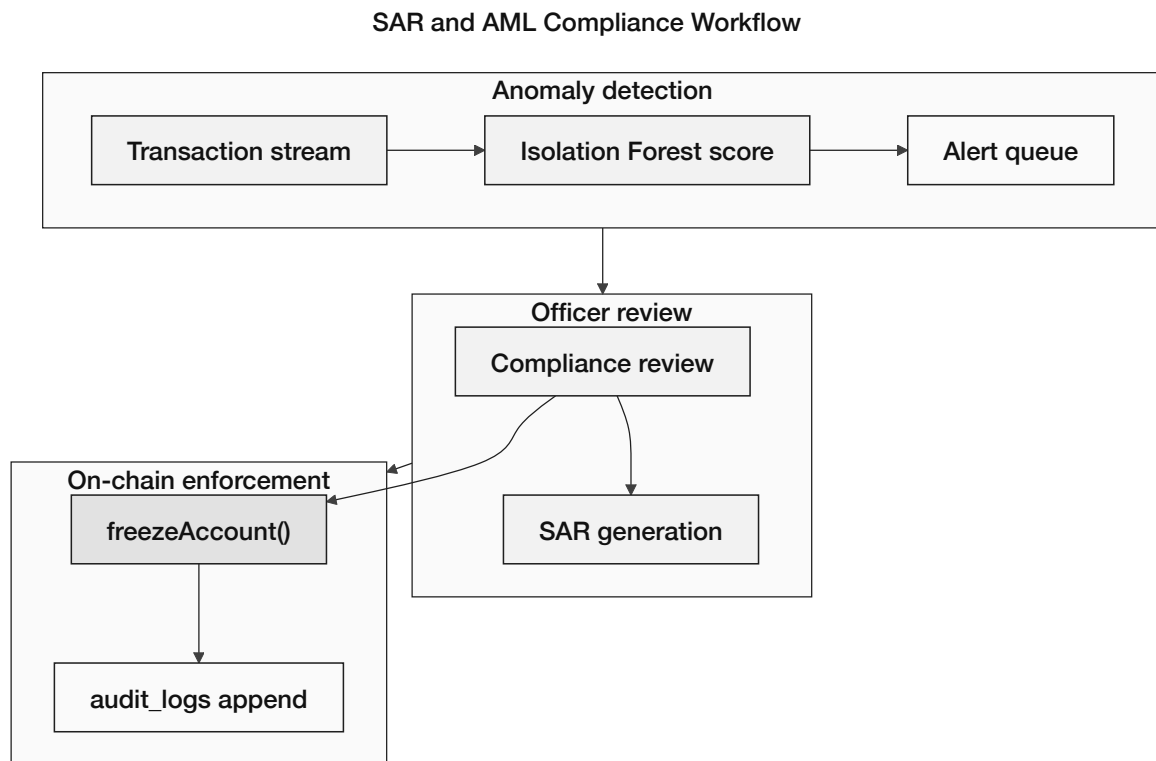
Figure 3.33: SAR and AML compliance workflow
