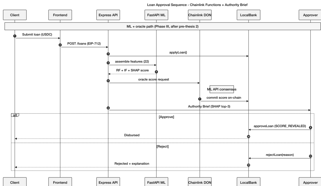
Figure 3.27: Loan approval sequence diagram
