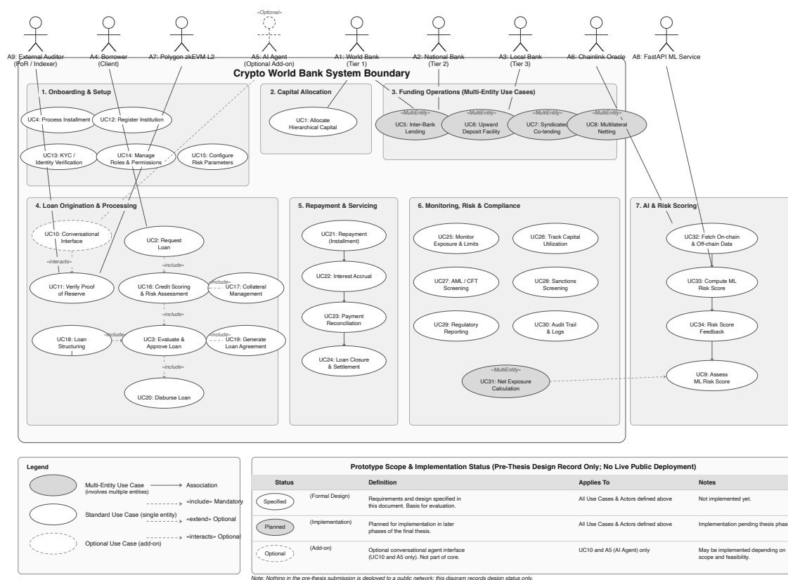
Figure 3.22: Use-case diagram (nine-actor taxonomy)
