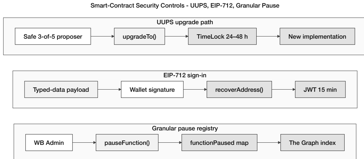
Figure 3.35: Smart-contract security controls
