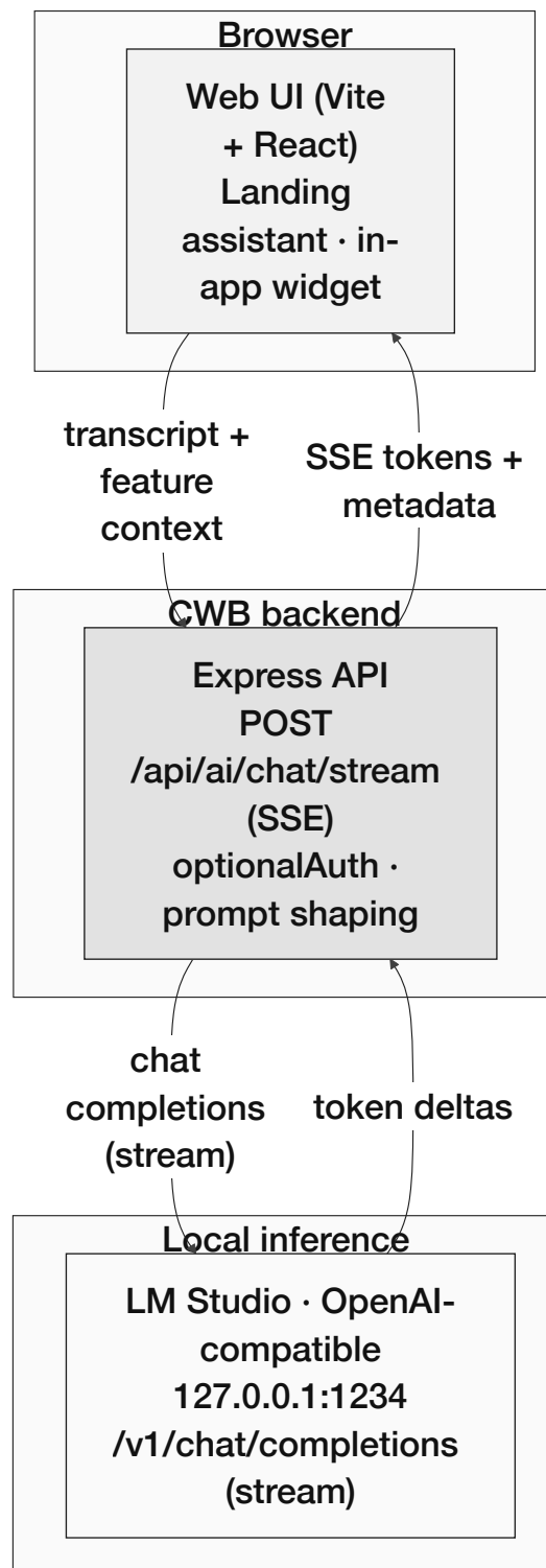
Figure 4.11: AI agent data flow (Phase III)
