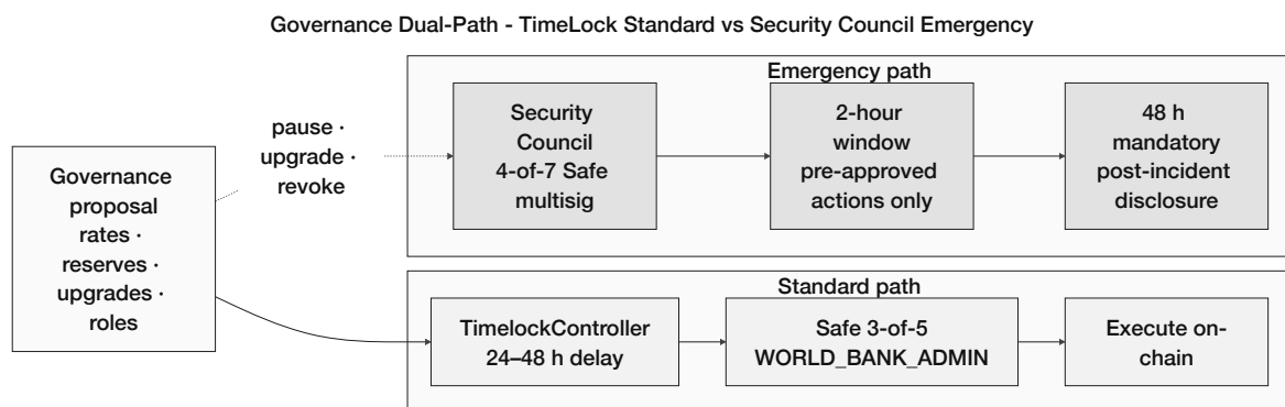
Figure 3.32: Governance dual-path
