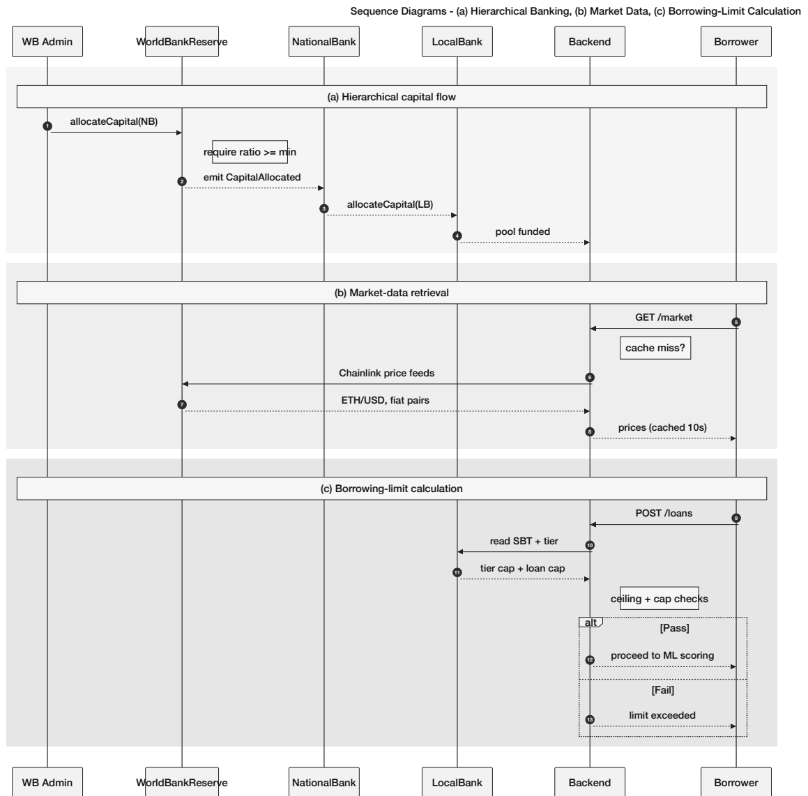
Figure 3.29: Sequence diagrams
