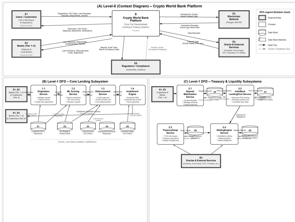
Figure 3.26: Data-flow diagrams
