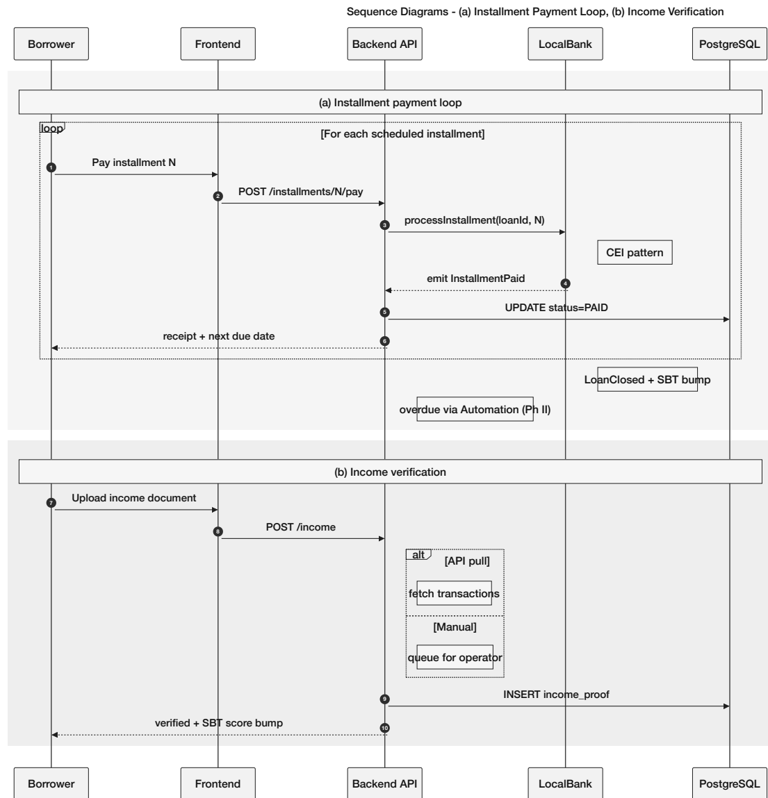
Figure 3.28: Sequence diagrams
