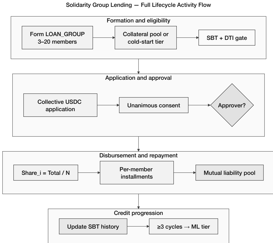
Figure 3.19: Solidarity group lending lifecycle (GroupLendingPool)
