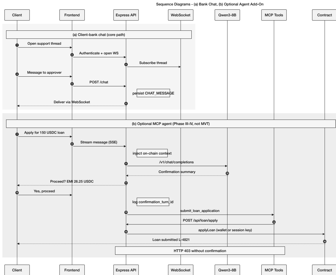
Figure 3.30: Sequence diagrams
